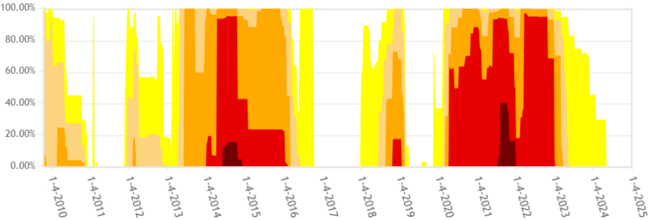
Figure 11:Siskiyou County Drought Conditions, U.S. Drought Monitor 2024.
