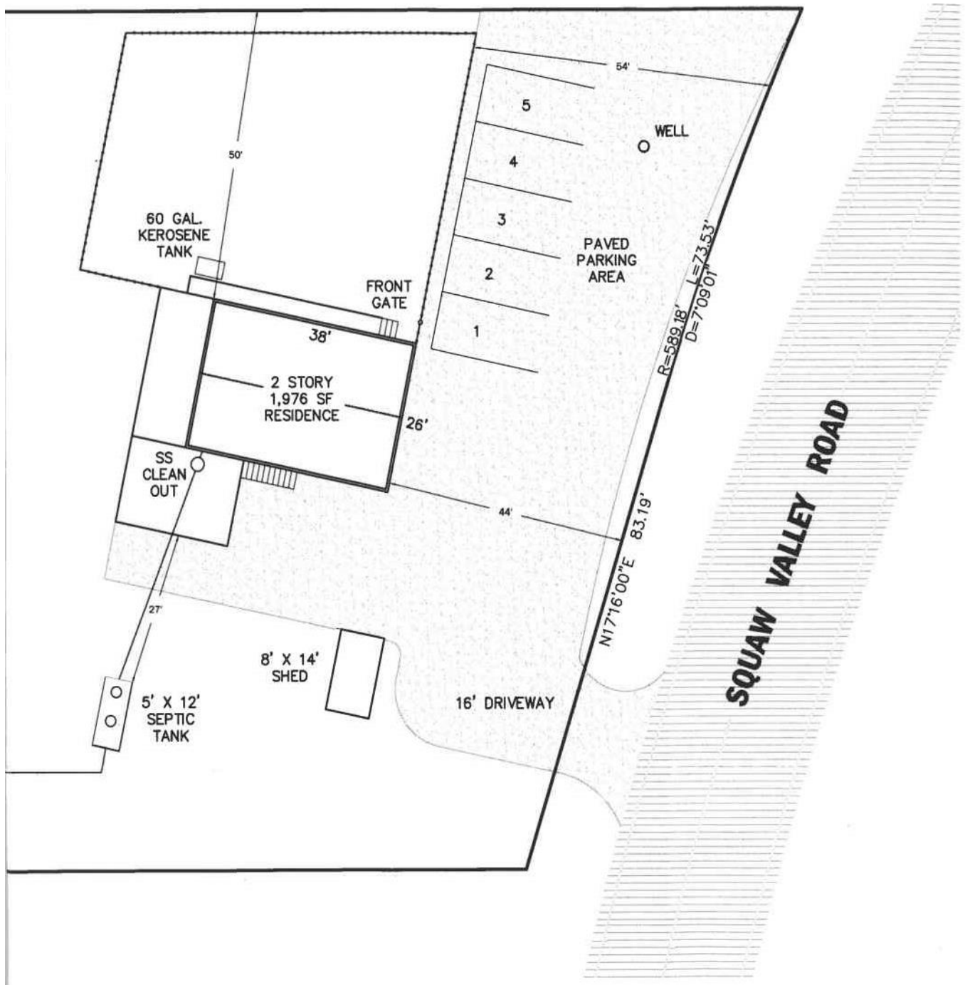
Figure 3: Site Plan
