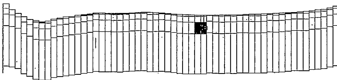
Figure 3. Cross-section of model grid in vicinity of well KVT1. Model rows are oriented along east-west cardinal directions on a compass: east is to the right and west is to the left.
