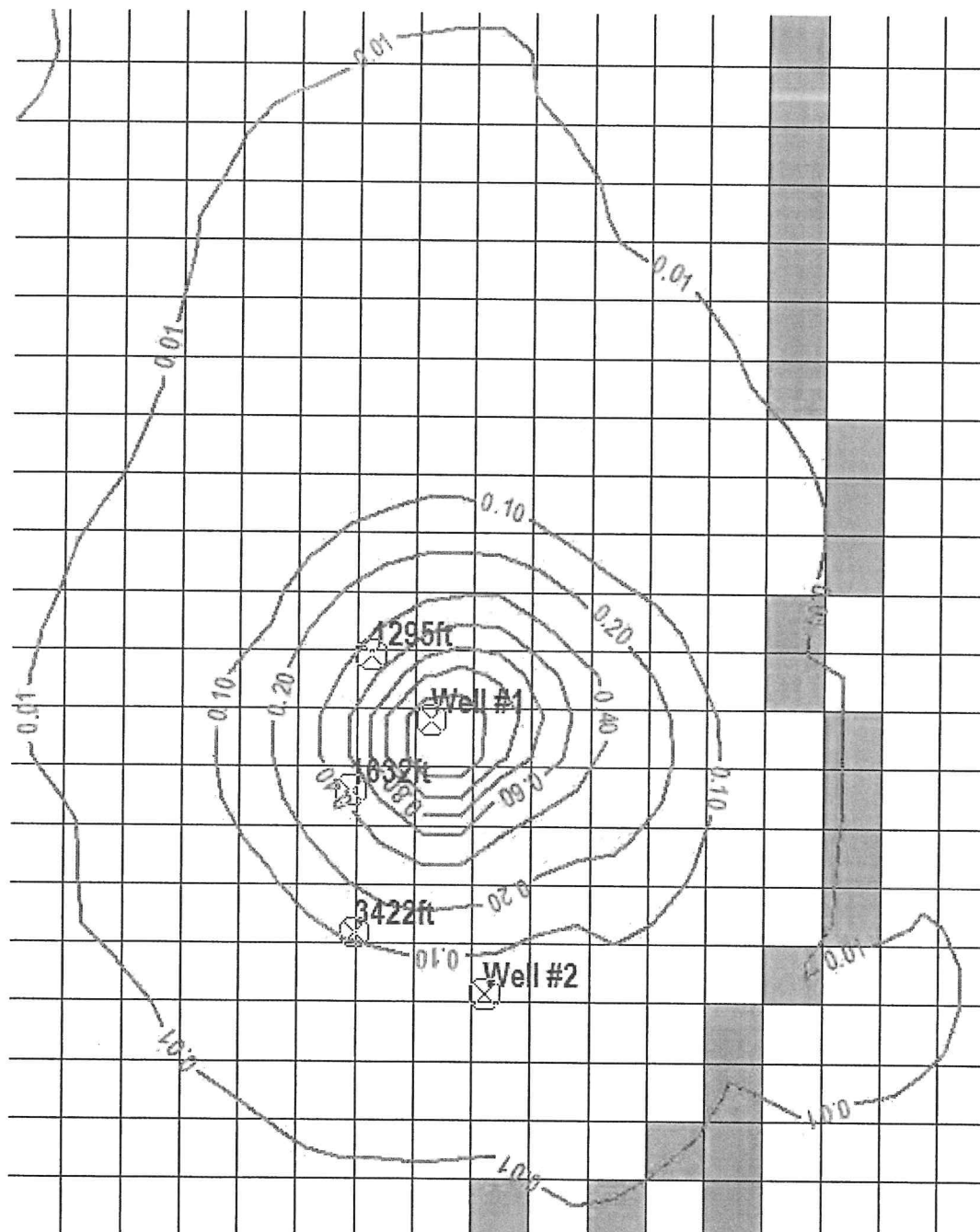
Figure 6. Drawdown Contours in Layer 1 (meters) Resulting from Pumping Well #1 for 60 days (contour interval varies)
