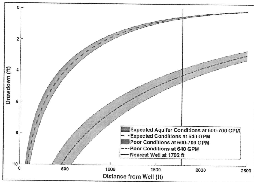
Figure 4. Simulated Seasonal Drawdown
