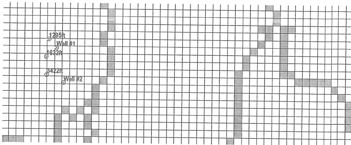
Figure 3. Model Grid and Nielsen Orchards Well Locations
